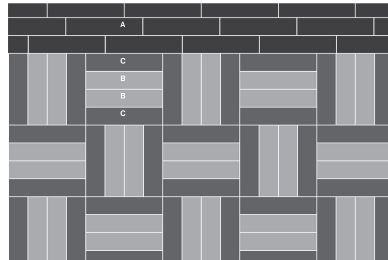
A CARPET TILE ON LINE SIZE 25CM X 1M COLOUR LIME INSTALLED ASHLAR B CARPET TILE FT510 SIZE 25CM X 1M COLOUR OCTAVE INSTALLED PATTERN BY TILE C CARPET TILE FT520 SIZE 25CM X 1M COLOUR OCTAVE INSTALLED PATTERN BY TILE
